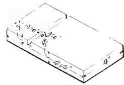
Fig. 2377. Stop block.
